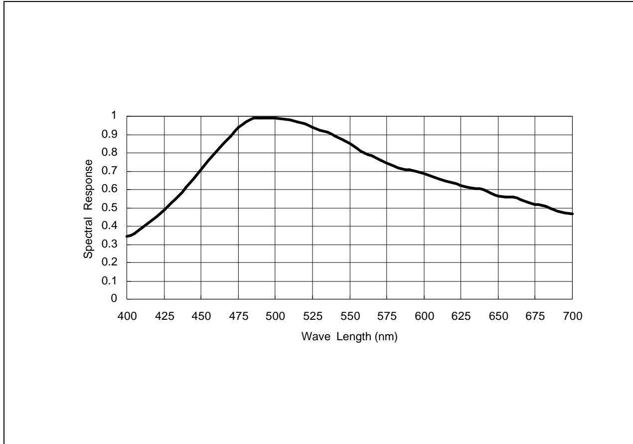
Figure 2. Spectral Response Characteristics
