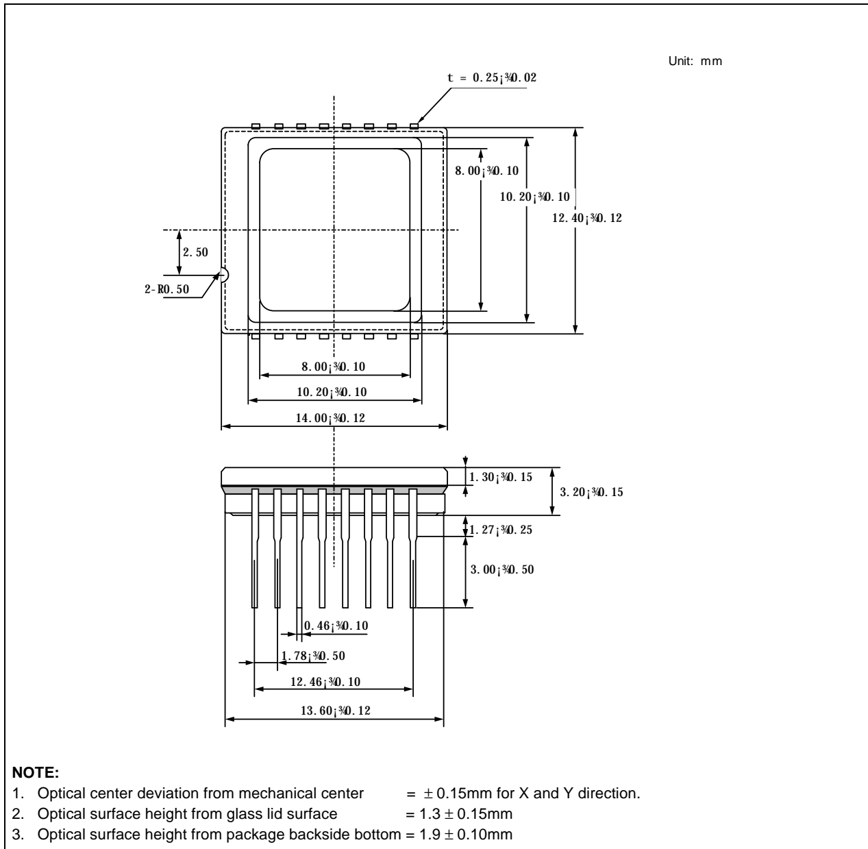
Figure 7. Package Dimensions
