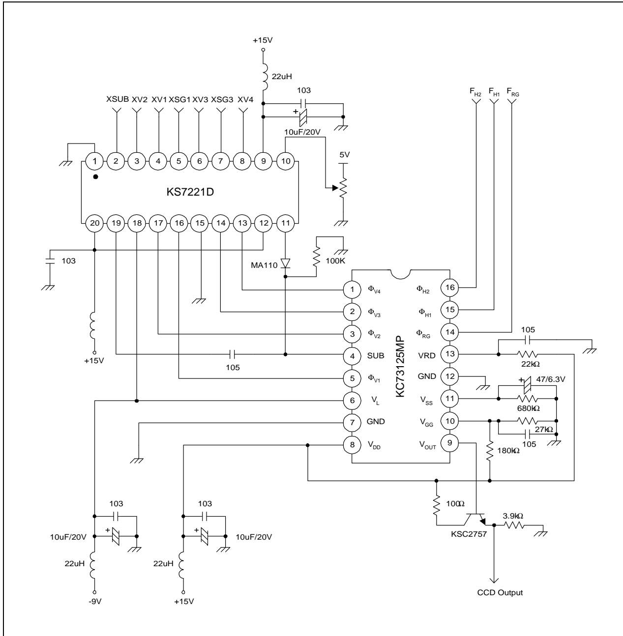
Figure 3. Application Circuits
