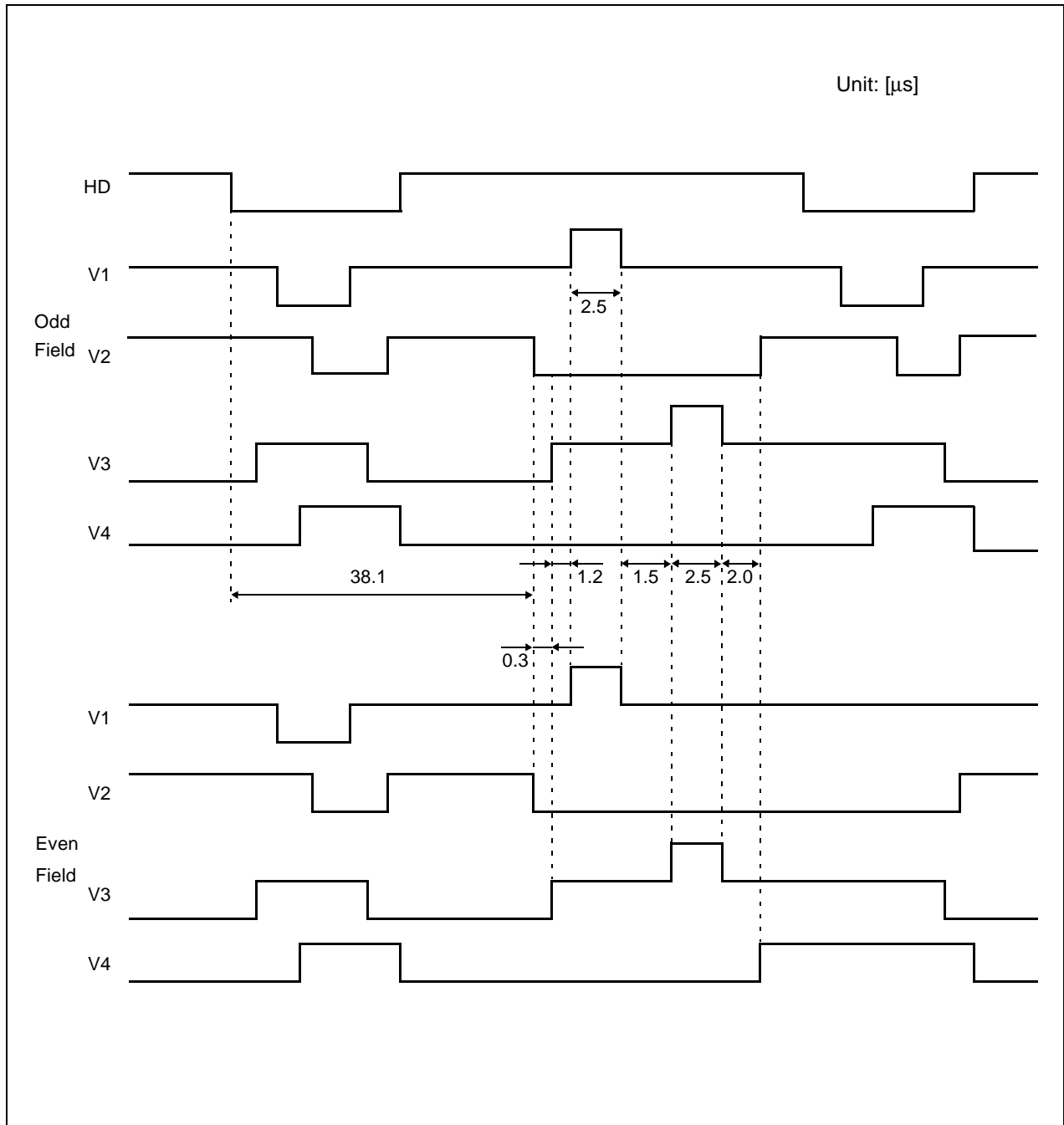
Figure 4. Read-out Clock Timing Chart
