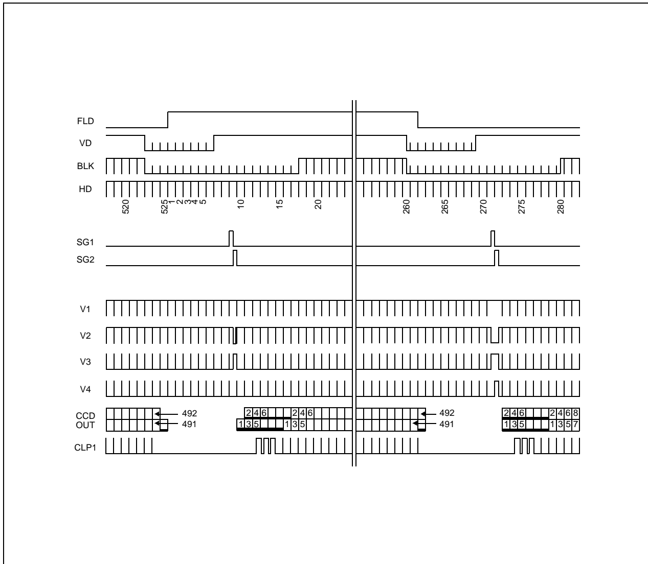
Figure 5. Clock Timing Chart (Vertical Sync.)
