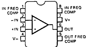
8-PIN MINI DIP (TOP VIEW) PACKAGE OUTLINE 9T PACKAGE CODE T
