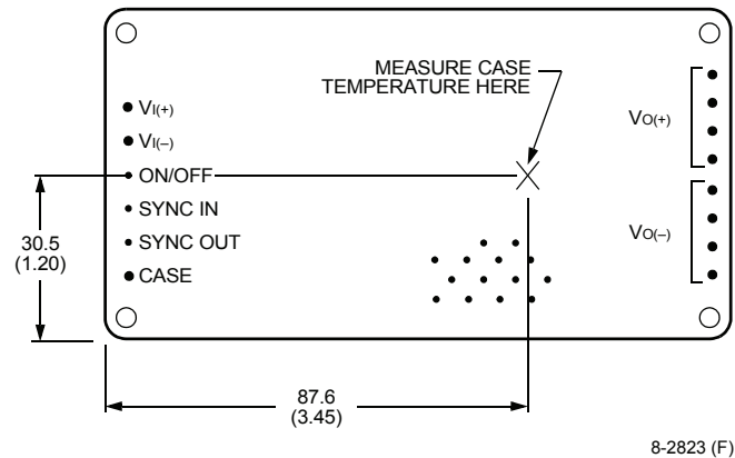
Note: Top view, measurements shown in millimeters and (inches). Pin locations are for reference only.
