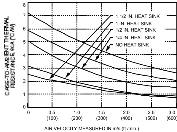
Figure 36. Case-to-Ambient Thermal Resistance Curves; Either Orientation
