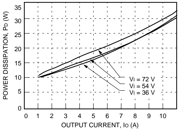
Figure 24. FW300R1 Power Dissipation vs. Output Current at 25 °C
