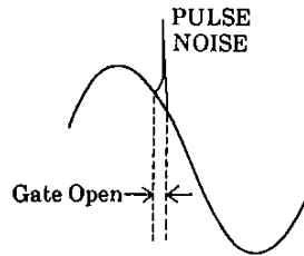
Noise canceller input waveform
