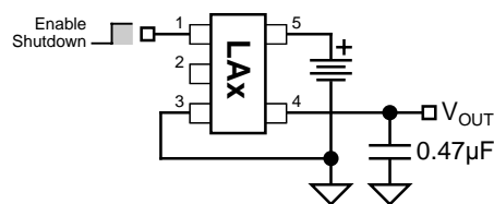
Regulator Circuit
