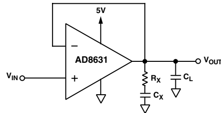
Figure 25. Snubber Network Compensation for Capacitive Loads
