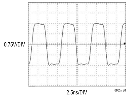
LTC6905-133 Output Operating at 133MHz, V_S = 3\text{V}
