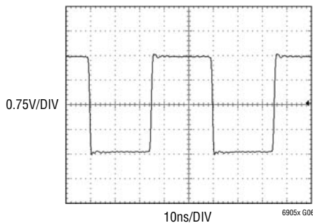
LTC6905-80 Output Operating at 20MHz, V_S = 3\text{V}
