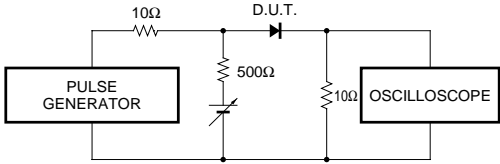
Fig.6 Reverse recovery time ( t_{rr} ) measurement circuit
