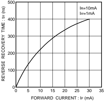
Fig.3 Reverse recovery time characteristics
