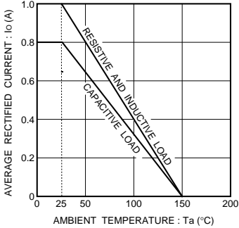
Fig.4 Derating curve
