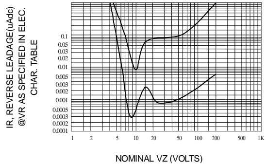
Fig. 4-TYPICAL REVERSE LEAKAGE
