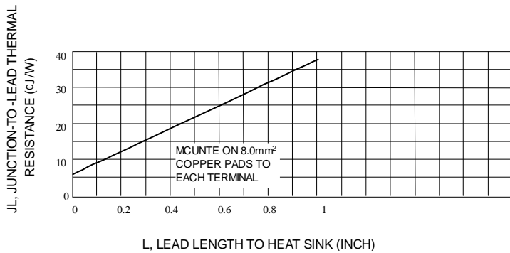
Fig. 4-TYPICAL THERMAL RESISTANCE
