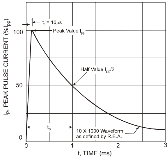
Fig. 3, Pulse Waveform
