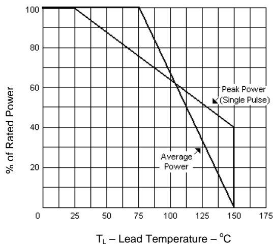
FIGURE 2 Lead Length = 3/8"
