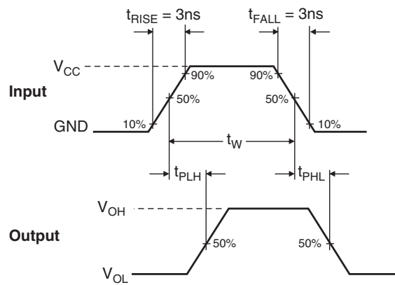
Figure 3. AC Waveforms
