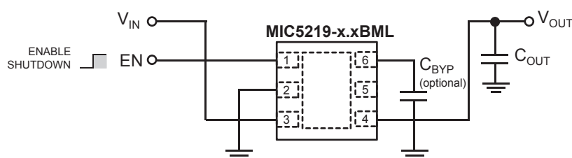
Ultra-Low-Noise Regulator
