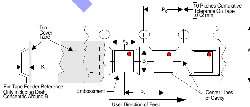
Figure 8. Tape and Reel Mechanical Data
