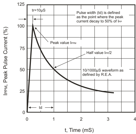
Fig.3 Pulse Waveform
