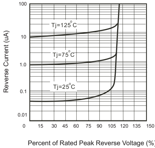
Fig. 1 - Reverse Characteristics
