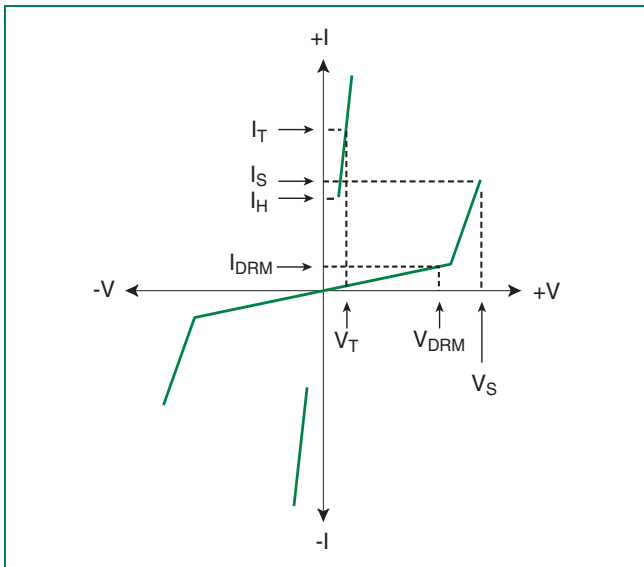
V-I Characteristics
