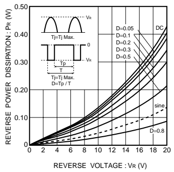
Fig. 7 Reverse power dissipation characteristics
