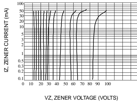
Fig. 8-VZ = 12 THRU 82 VOLTS
