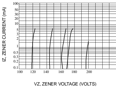
Fig. 9-VZ = 100 THRU 200 VOLTS
