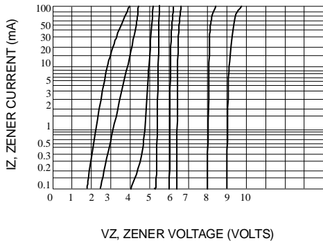
Fig. 7-VZ = 3.9 THRU 10 VOLTS
