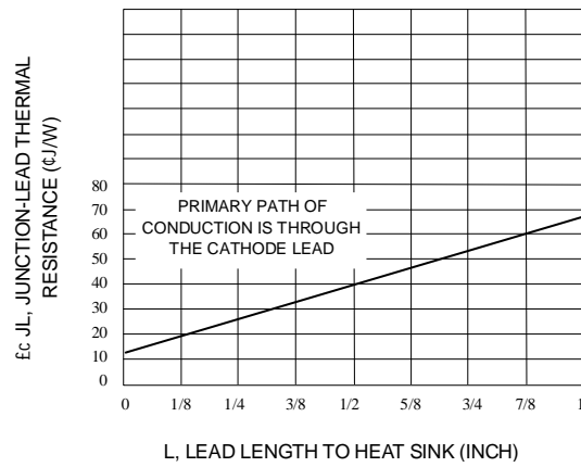
Fig. 10-TYPICAL THERMAL RESISTANCE
