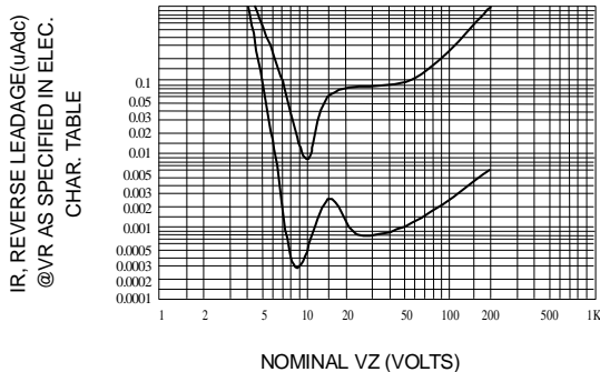
Fig. 4-TYPICAL REVERSE LEAKAGE
