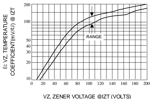
Fig. 6-UNITS 10 TO 200 VOLTS
