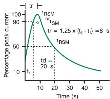
8/20μS IMPULSE DISCHARGE CURRENT WAVESHAVE
