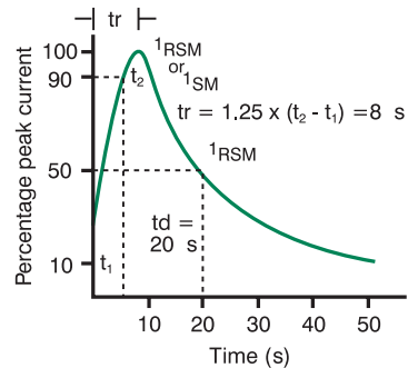
8/20 \mu S IMPULSE DISCHARGE CURRENT WAVESHAP
