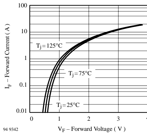
Figure 3. Max. Forward Current vs. Forward Voltage
