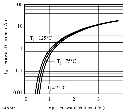
Figure 3. Max. Forward Current vs. Forward Voltage
