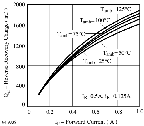
Figure 5. Typ. Reverse Recovery Charge vs. Forward Current
