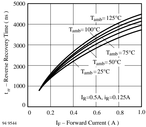
94 9544 I_F – Forward Current (A) Figure 4. Typ. Reverse Recovery Time vs. Forward Current
