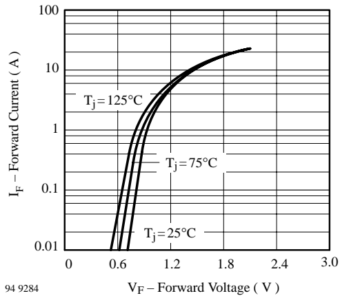
94 9284 V_F – Forward Voltage (V) Figure 3. Typ. Forward Current vs. Forward Voltage
