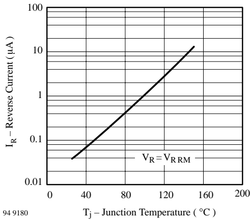
94 9180 T_j – Junction Temperature ( ^\circ\text{C} ) Figure 1. Typ. Reverse Current vs. Junction Temperature
