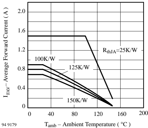
94 9179 T_{amb} – Ambient Temperature ( ^\circ\text{C} ) Figure 2. Max. Average Forward Current vs. Ambient Temperature
