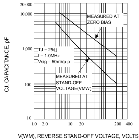
Fig. 4-TYPICAL JUNCTION CAPACITANCE
