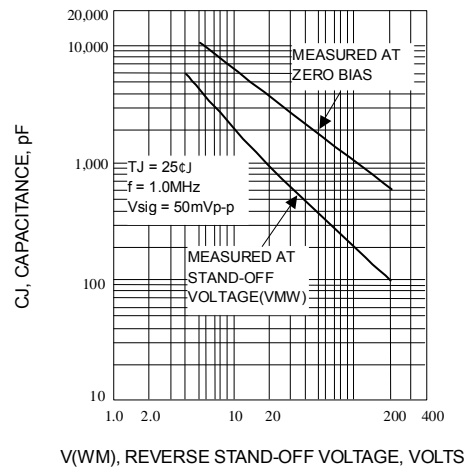
Fig. 4-TYPICAL JUNCTION CAPACITANCE
