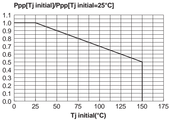
Fig. 1: Peak power dissipation versus initial junction temperature.
