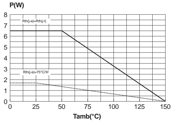
Fig. 2: Continuous power dissipation versus initial junction temperature.
