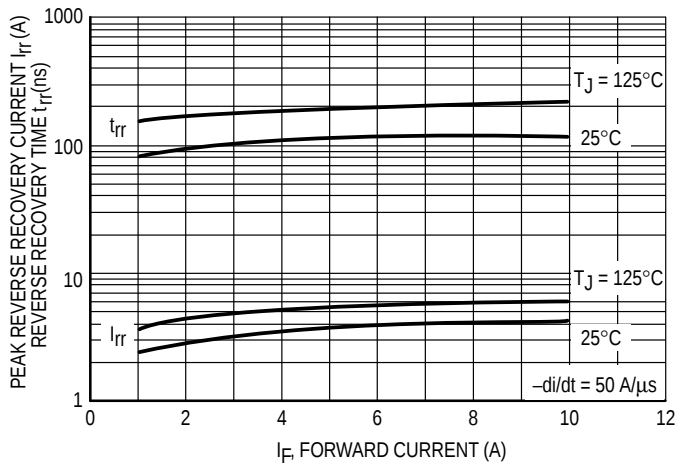
Figure 4. Output Inverter Reverse Recovery t_{rr} , I_{rr} versus Forward Current I_F
