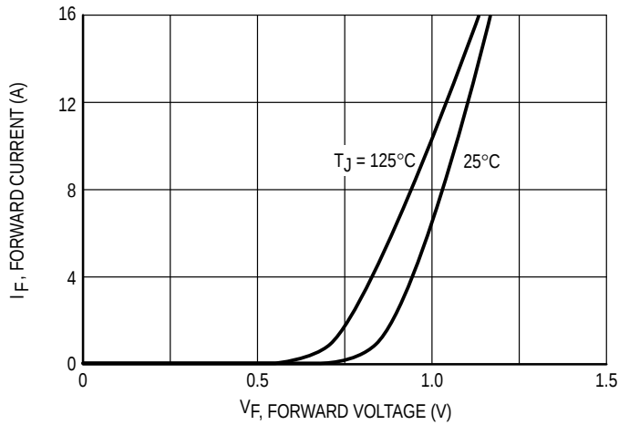
Figure 2. Input Bridge Forward Current I_F versus Forward Voltage V_F
