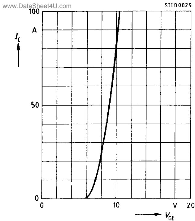
Typ. transfer characteristics I_C = f(V_{GE}) parameter: t_p = 80 \text{ } \mu\text{s}, V_{CE} = 20 \text{ V}
