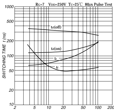
Fig. 7 Typical Switching Time Vs. Drain Current
