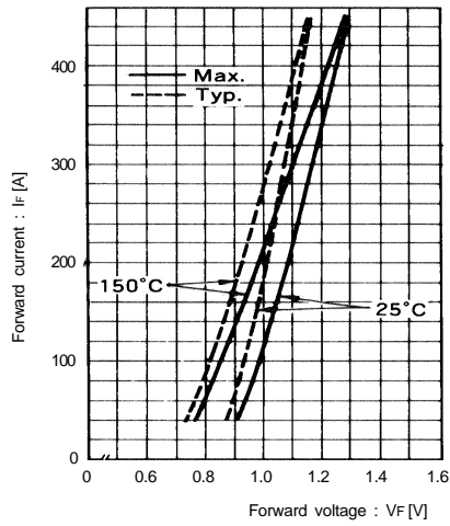
Forward Characteristics
