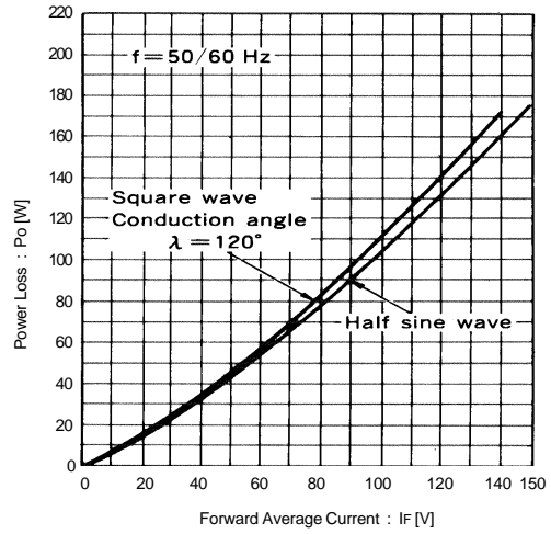
Forward Average Current vs. Power Loss
