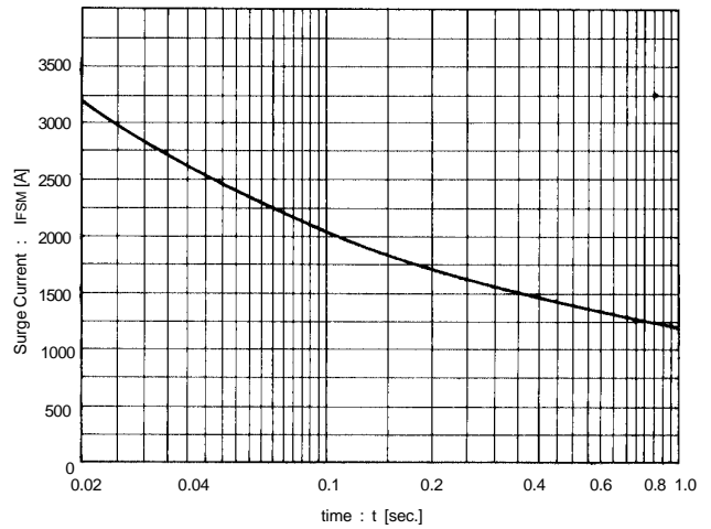
Surge Current
