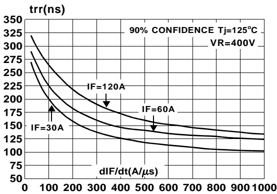
Fig. 5: Reverse recovery time versus dI/dt.
