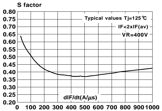
Fig. 6: Softness factor (tb/ta) versus dI/dt.
