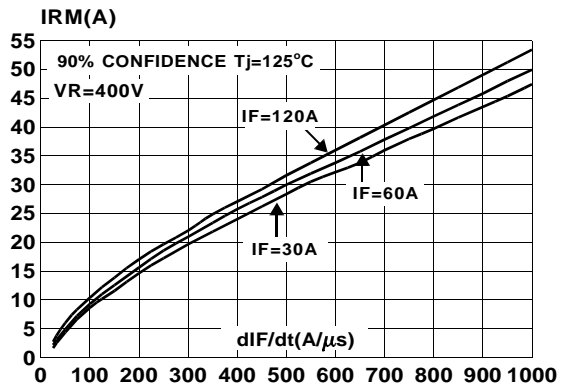
Fig. 4: Peak reverse recovery current versus dI/dt.
