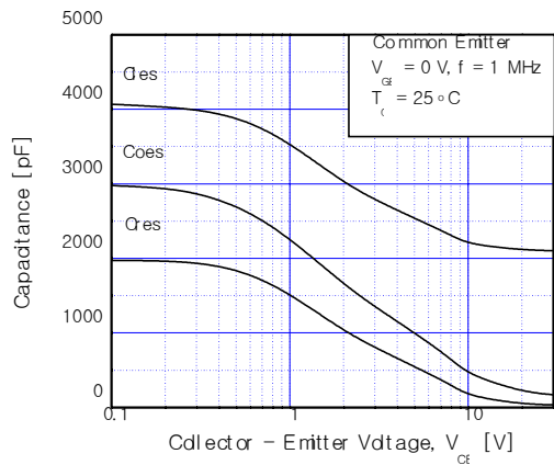
Fig 6. Capacitance Characteristics
