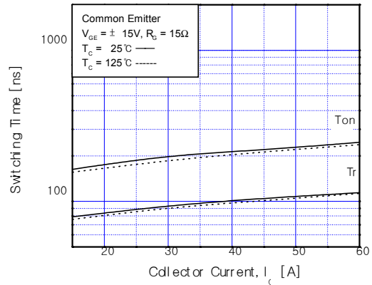
Fig 10. Turn-On Characteristics vs. Collector Current
