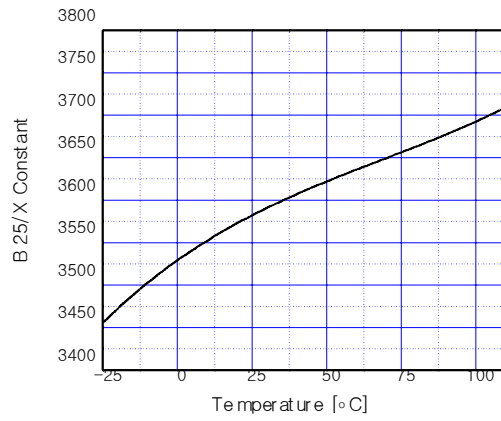
Fig 20. NTC Characteristics
