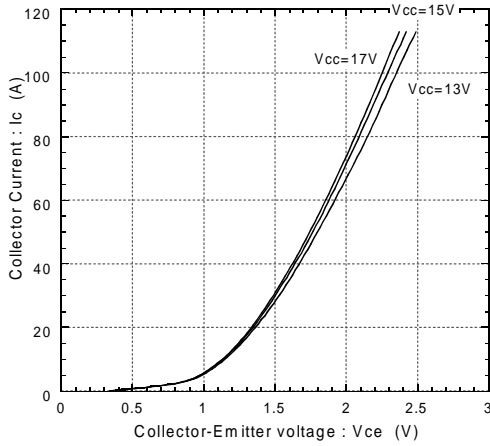
Collector current vs. Collector-Emittter voltage Tj=25°C
