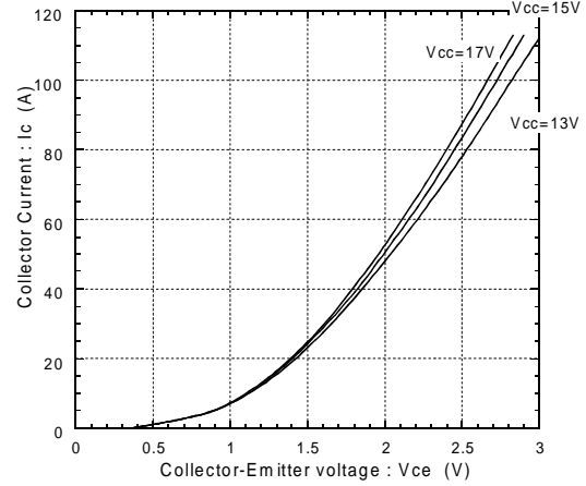
Collector current vs. Collector-Emittter voltage Tj=125°C
