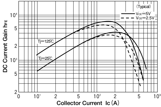
D.C. Current Gain
