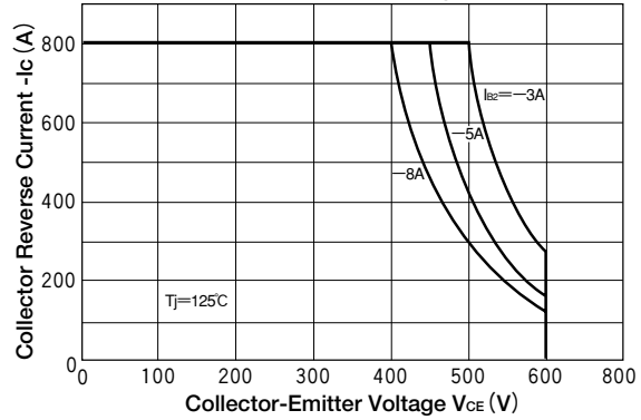
Reverse Bias Safe Operating Area
