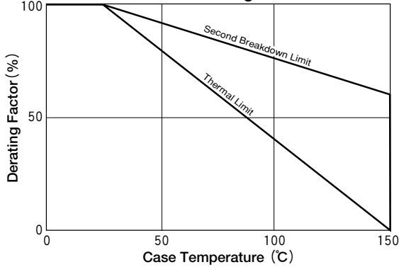
Collector Current Derating Factor
