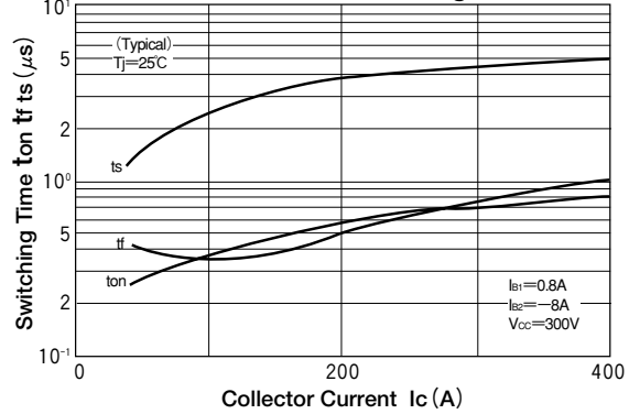
Collector Current Vs Switching Time
