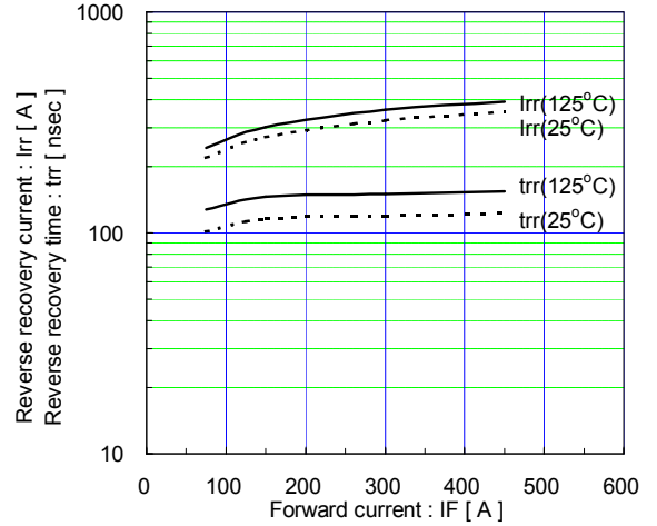
Reverse recovery characteristics (typ.) Vcc=600V, VGE=±15V, RG=1.1Ω
