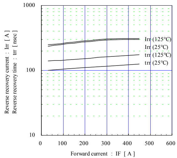
Reverse recovery characteristics (typ.) Vcc=600V, VGE=±15V, Rg=1.1Ω
