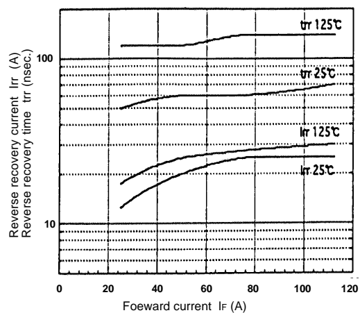
Reverse recovery characteristics trr, Irr, vs. If
