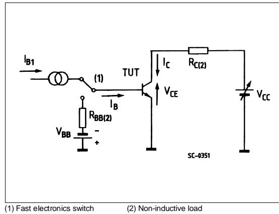
(1) Fast electronics switch (2) Non-inductive load
