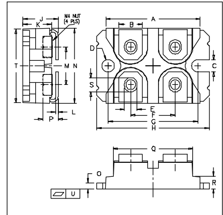
Package Outline
