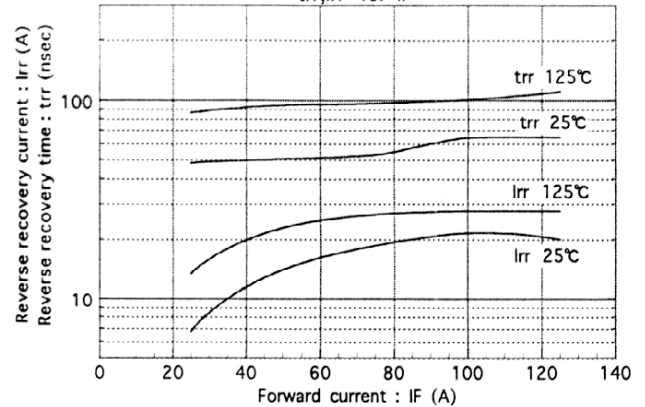
Reverse recovery characteristics trr, Irr vs. IF
