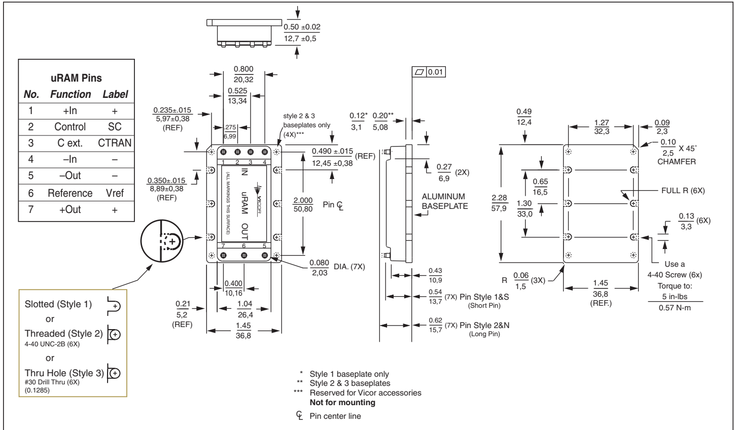
Figure 17 — Module outline
