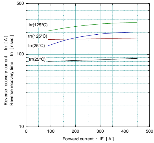
Reverse recovery characteristics (typ.) Vcc=600V, VGE=+15V, Rg=2.7ohm
