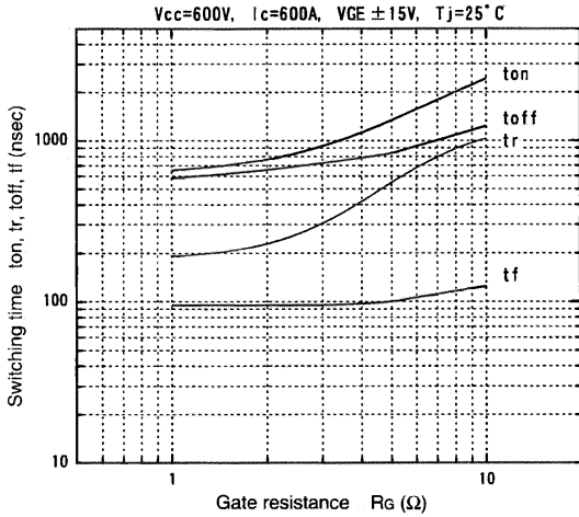
Switching time vs. Gate resistance
